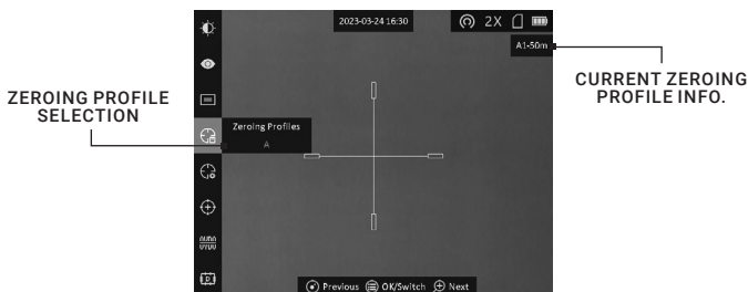
FIGURE 2-7. ZEROING PROFILES
