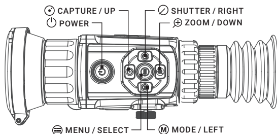
FIGURE 2-2. CONTROL BUTTONS
