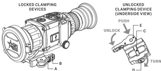
FIGURE 2-5. MOUNT
