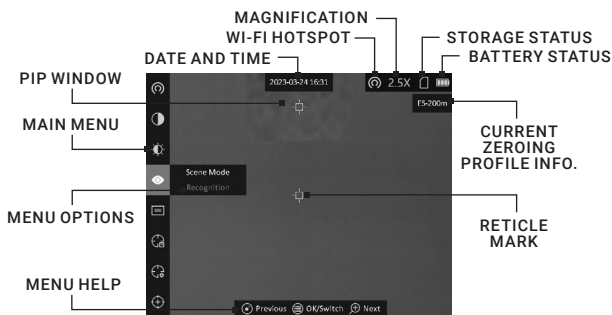
FIGURE 2-3. ON-SCREEN DISPLAY
