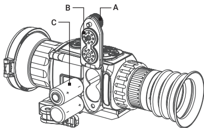
FIGURE 2-1. BATTERY INSTALLATION
