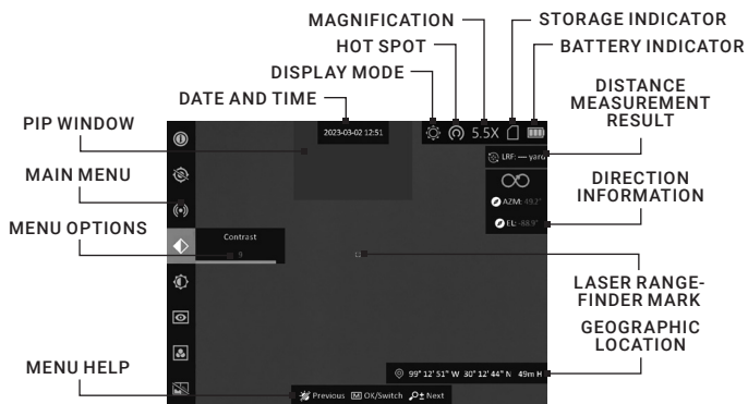
FIGURE 2-3. ON-SCREEN DISPLAY
